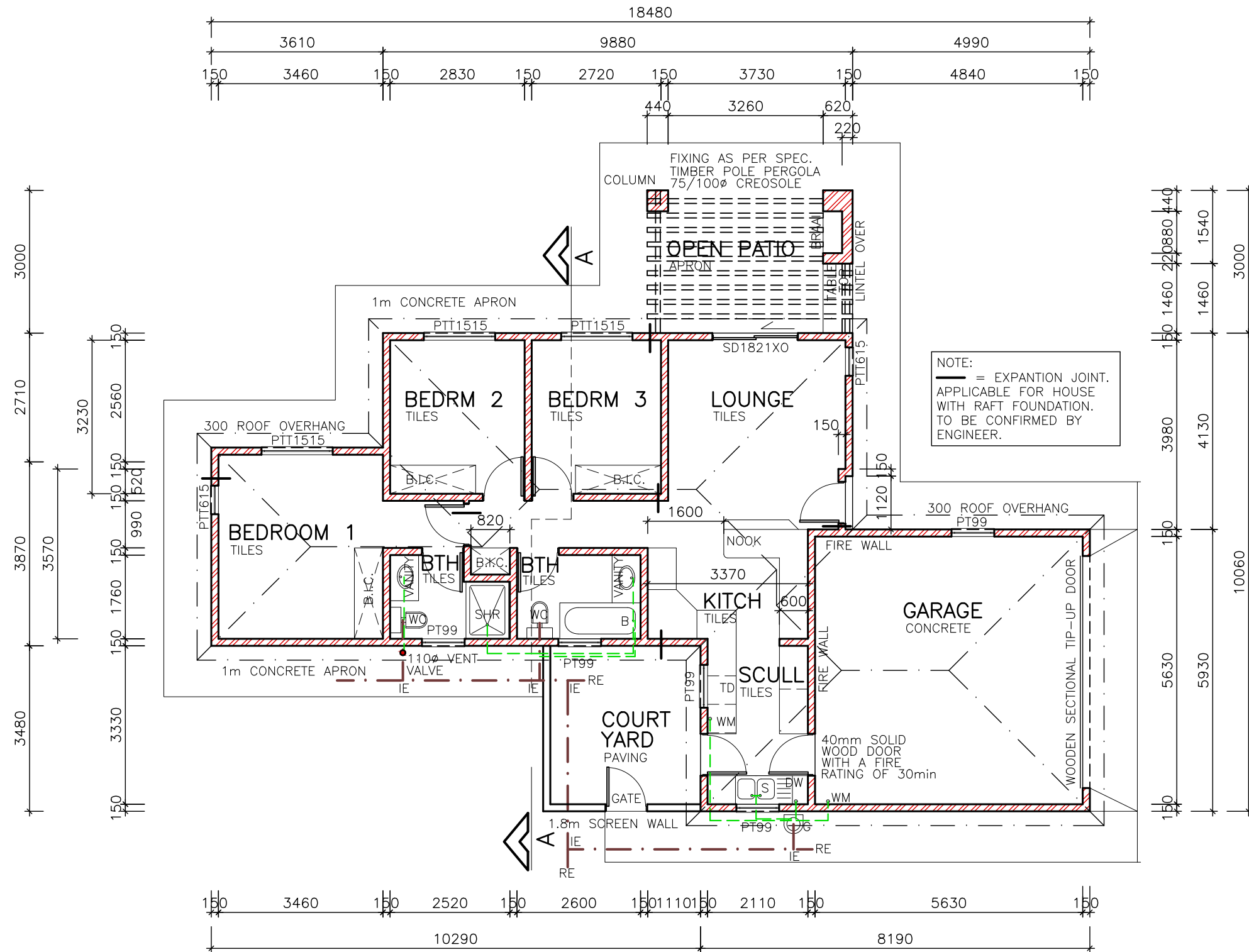
PLAN SCALE 1:100
