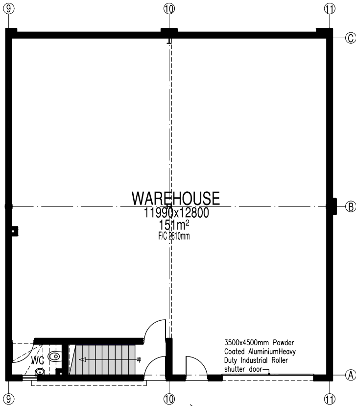
GROUND STOREY NOT TO SCALE
