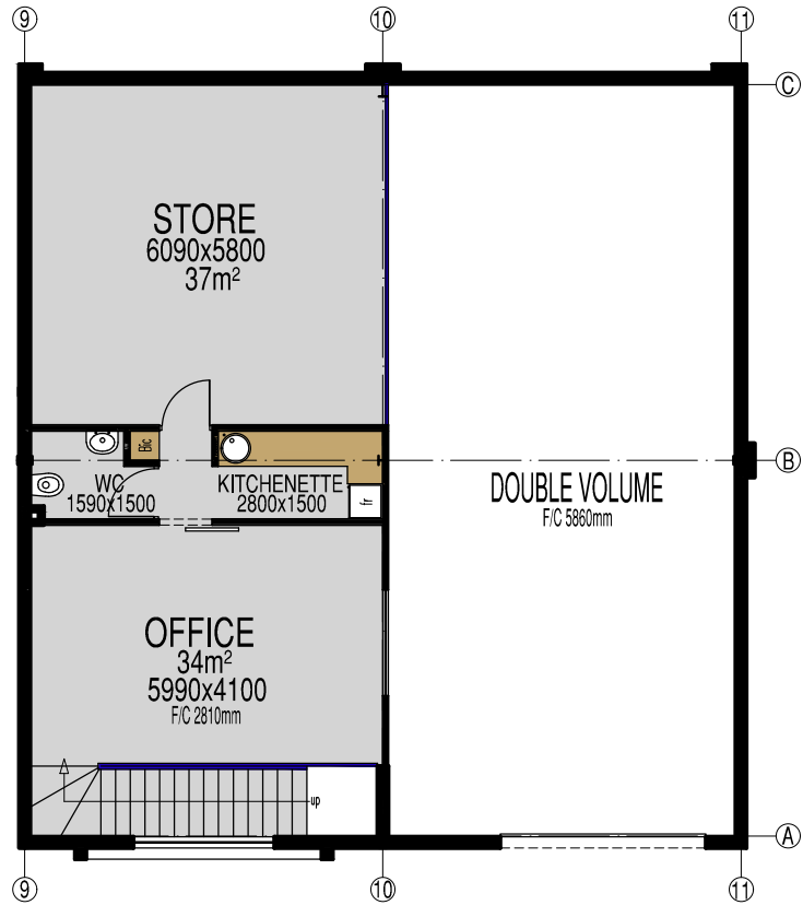
FIRST STOREY NOT TO SCALE
