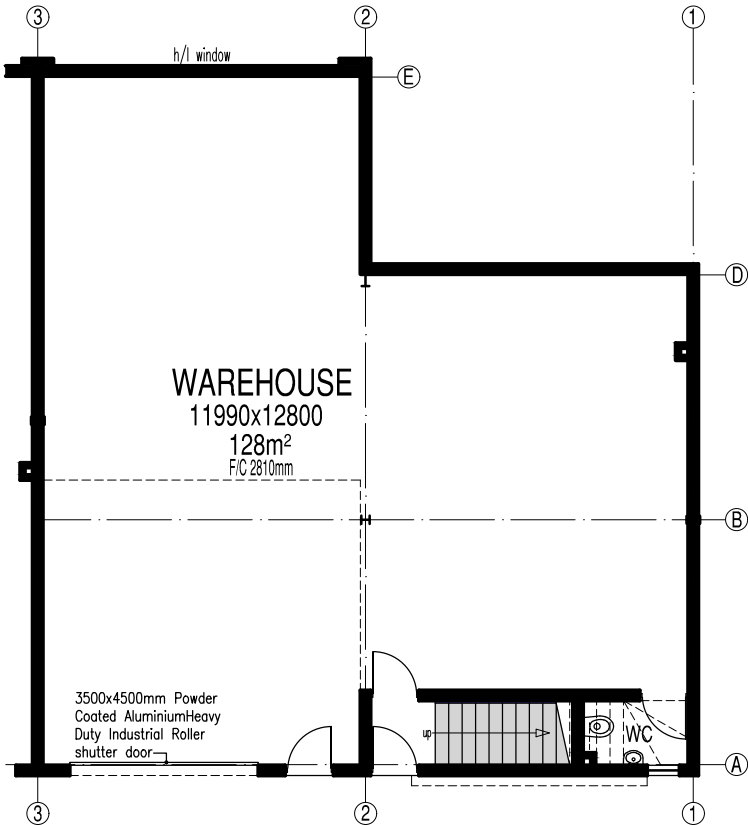
GROUND STOREY NOT TO SCALE
