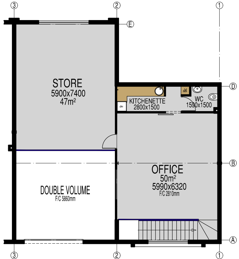
FIRST STOREY NOT TO SCALE
